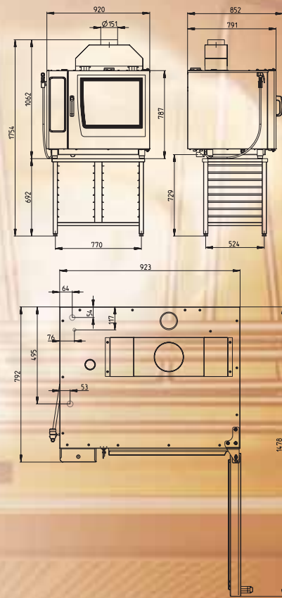
Gas combi oven 6 x GN1/1 – pg, sg, cg
