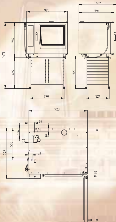
Electric combi oven 6 x GN1/1 – pi, si, ci, pb, sb, cb
